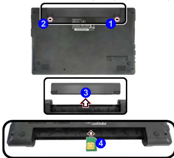
Figure 6 - 15 USIM Card Insertion
